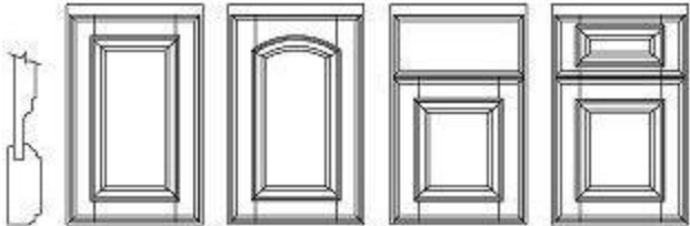
RAISED PANEL - FULL OVERLAY
